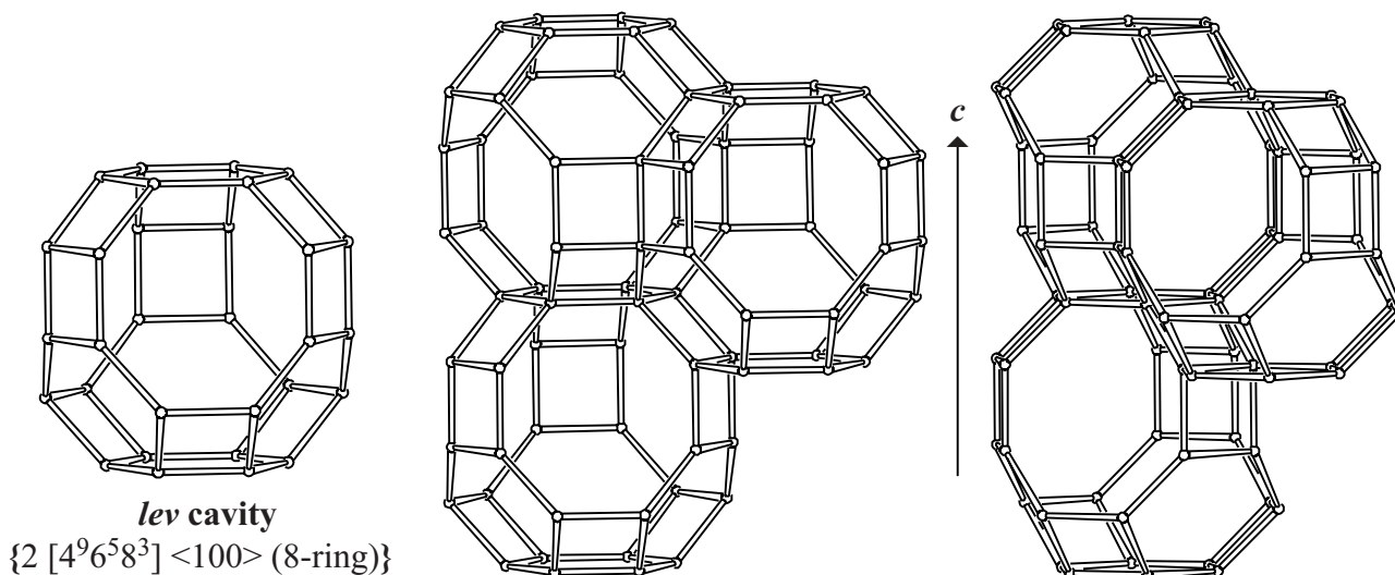
Figure 4. lev Cavity (left) and fused cavities (middle) viewed along \langle 120 \rangle and fused cavities viewed along \langle 100 \rangle (right). ▲
