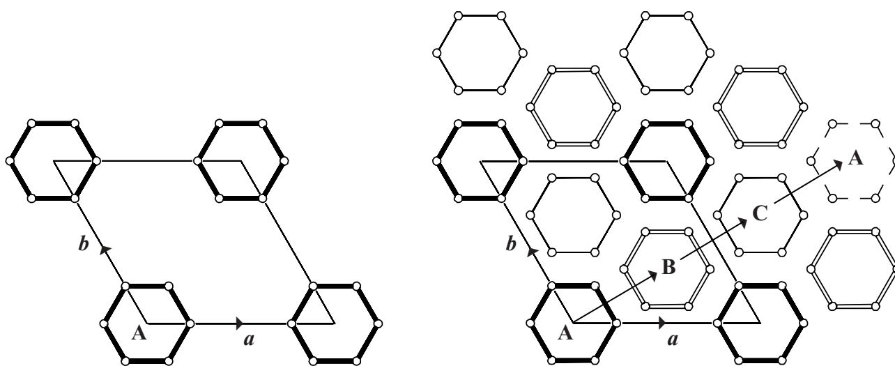
Figure 1: PerBU in LEV (left) and definition of 6-ring positions with respect to each other (right).
