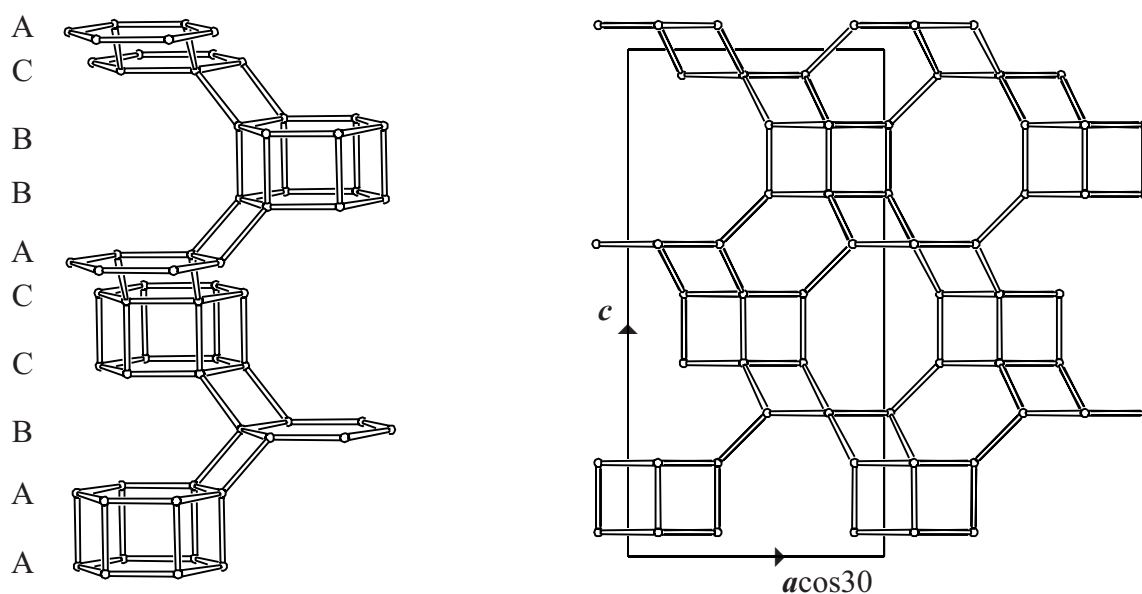
Figure 3. Perspective drawing (left) and projection of the unit cell content (right) along b . The stacking sequence is given. In the perspective drawing each PerBU is represented by one 6-ring. ▲
