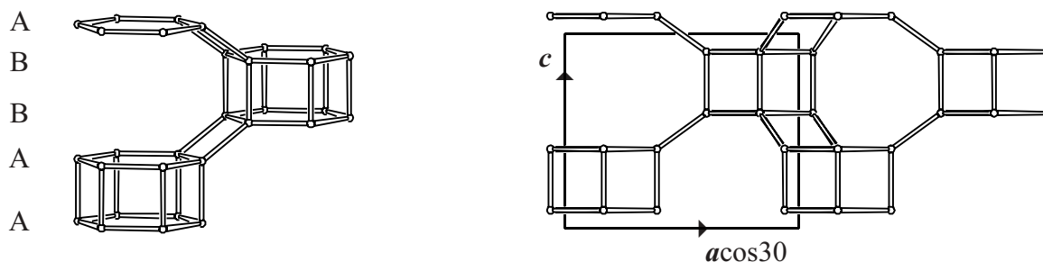
Figure 3. Perspective drawing (left) and projection of the unit cell content (right) along b . The stacking sequence is given. In the perspective drawing each PerBU is represented by one 6-ring. [GME can also be built using double 6-rings, or 4-rings or 4-2 units; see Alternative description ].
