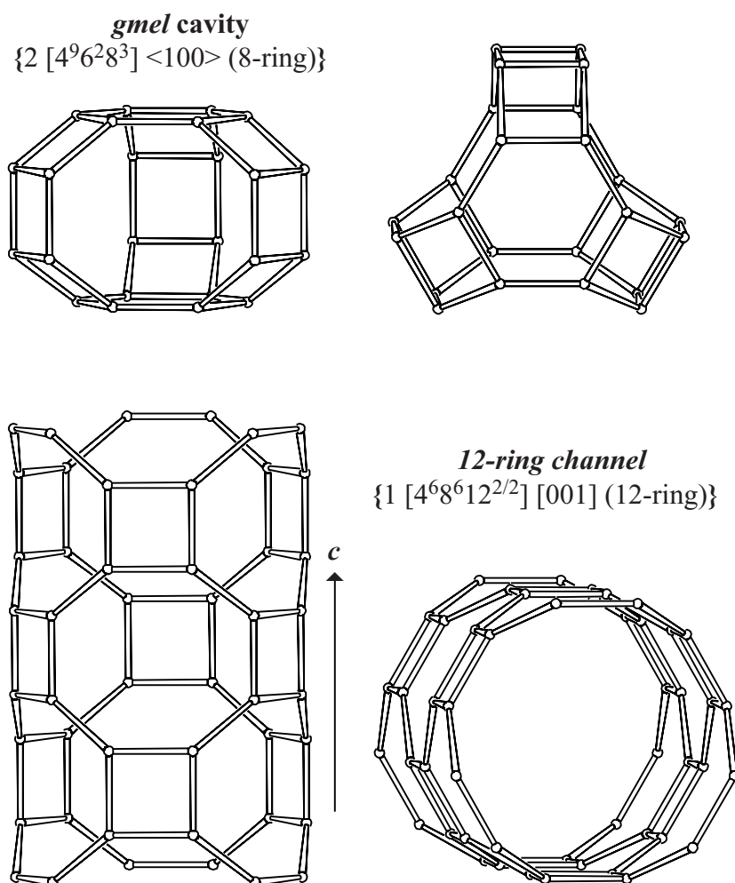
Figure 4. gmel Cavity (top) and 12-ring channel (bottom) viewed along \langle 120 \rangle (left), and along c (right). The pure descriptors are added. [Figure 5 is on next page]
