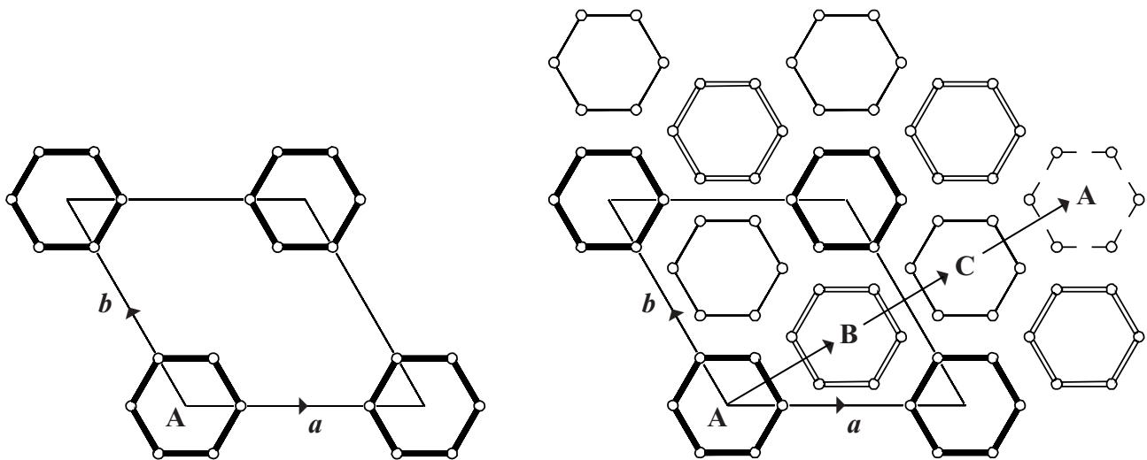
Figure 1: PerBU in GME (left) and definition of 6-ring positions with respect to each other (right).
