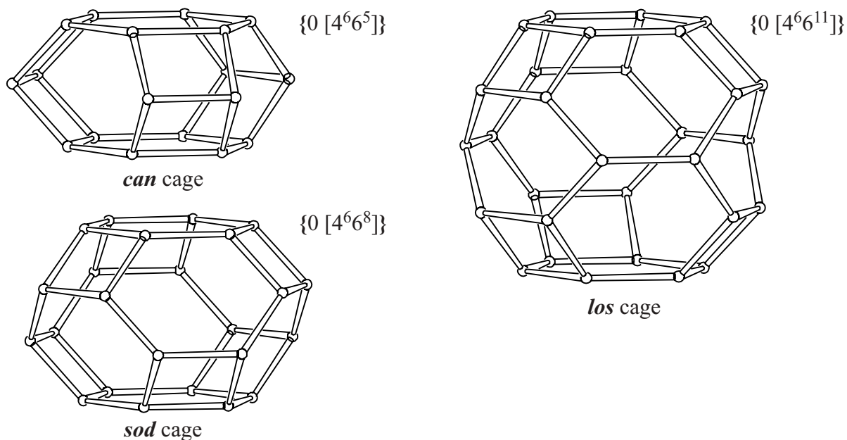
Figure 4. can Cage, (or \epsilon -cage; top left), sod cage (or \beta -cage; bottom left) and los cage (right) viewed perpendicular c . [Figure 5 is on next page]
