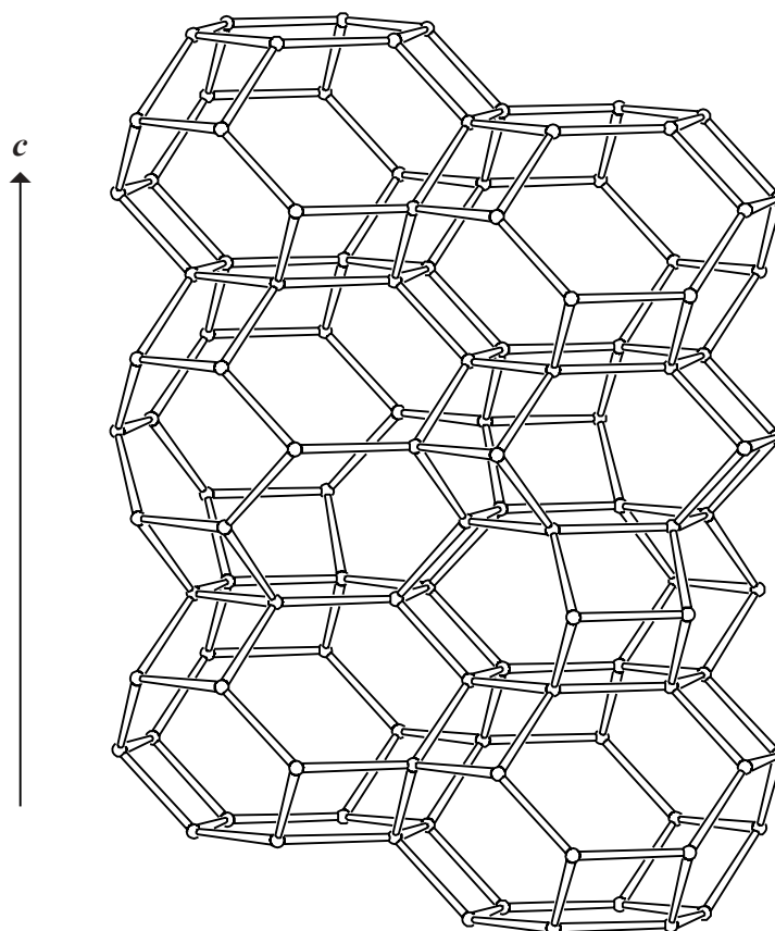
Figure 5. Fused cages, (viewed perpendicular to c ), form "channels" with 6-ring apertures. ▲
