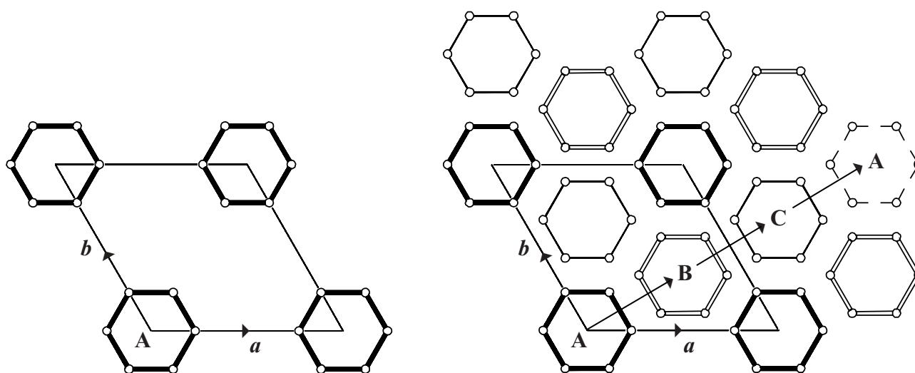
Figure 1: PerBU in FRA (left) and definition of 6-ring positions with respect to each other (right).
