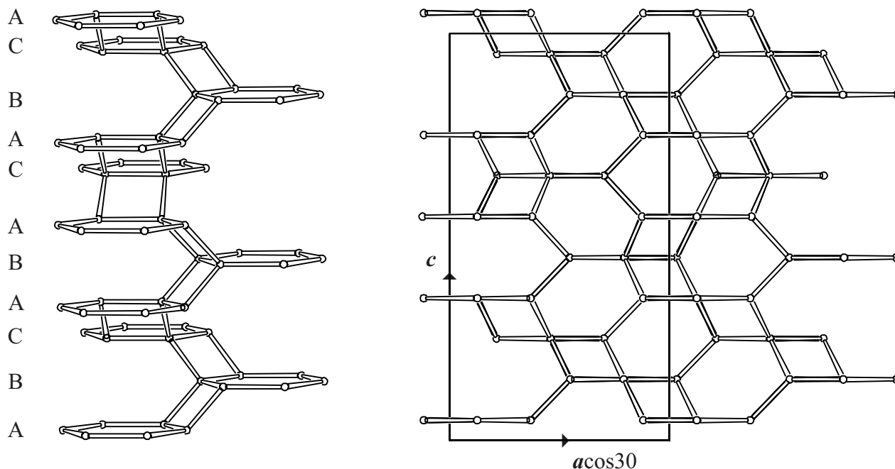
Figure 3. Perspective drawing (left) and projection of the unit cell content (right) along b . The stacking sequence is given. In the perspective drawing each PerBU is represented by one 6-ring. [FRA can also be built using 4-rings] ▲
