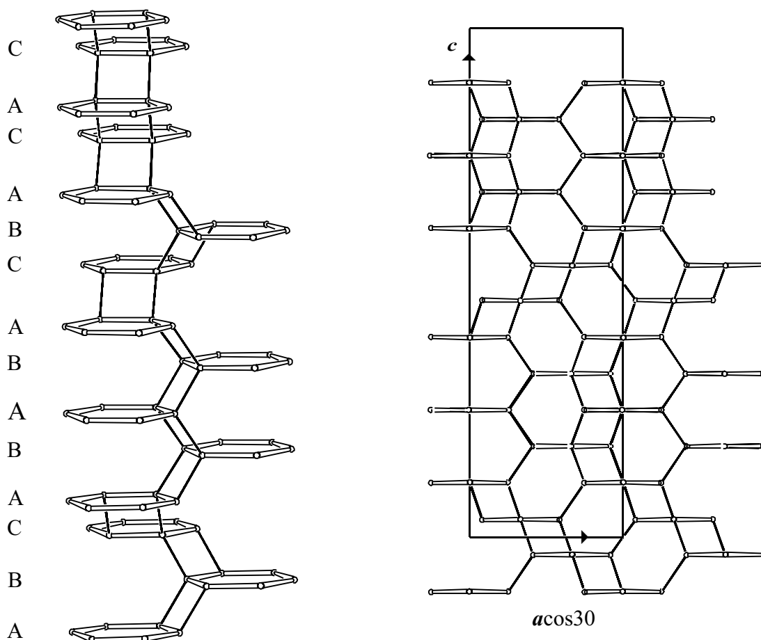
Figure 3. Perspective drawing (left) and projection of the unit cell content (right) along b . The stacking sequence is given. In the perspective drawing each PerBU is represented by one 6-ring. ▲
