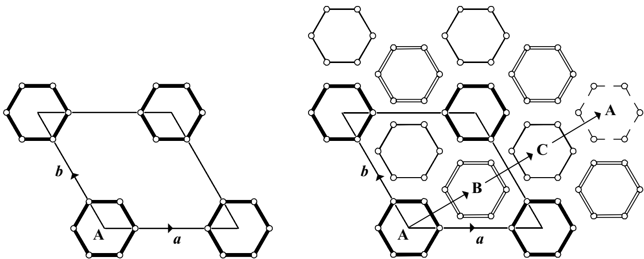
Figure 1: PerBU in FAR (left) and definition of 6-ring positions with respect to each other (right).
