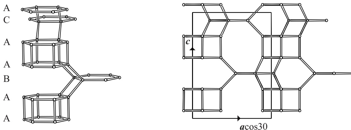
Figure 3. Perspective drawing (left) and projection of the unit cell content (right) along b . The stacking sequence is given. In the perspective drawing each PerBU is represented by one 6-ring. [ERI can also be built using 4-rings]
