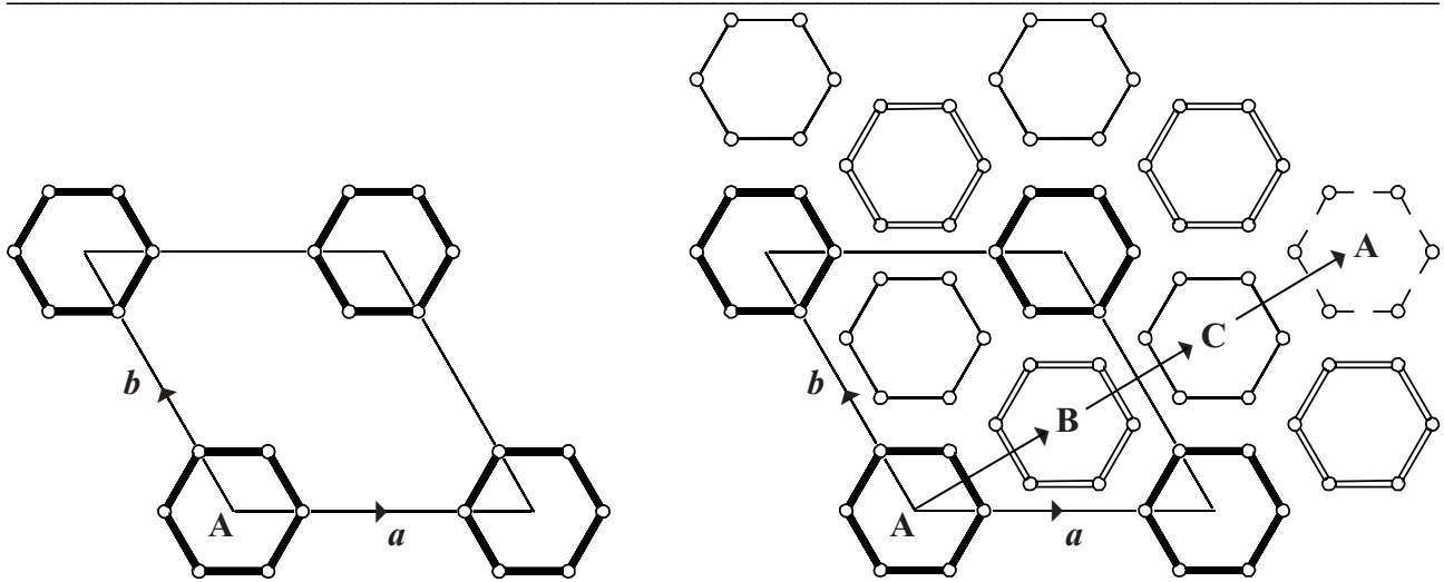
Figure 1: PerBU in ERI (left) and definition of 6-ring positions with respect to each other (right).
