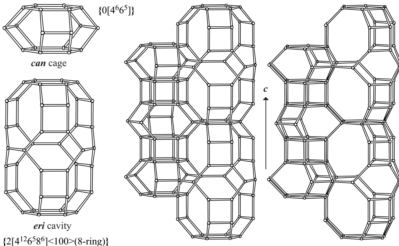
Figure 4. can Cage (top left) and eri cavity (bottom left) viewed along \langle 120 \rangle , fused cages viewed along \langle 120 \rangle (middle) and 8-ring channels viewed along \langle 100 \rangle (right).
