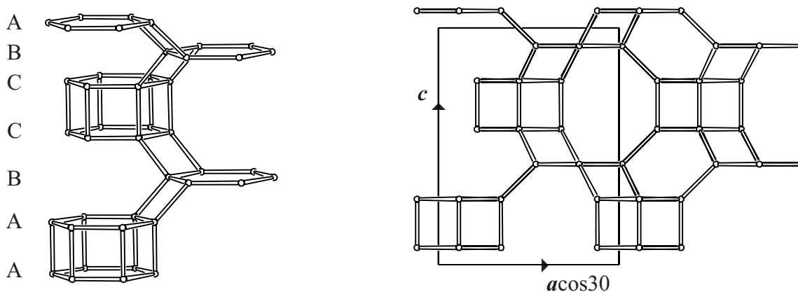
Figure 3. Perspective drawing (left) and projection of the unit cell content (right) along b . The stacking sequence is given. In the perspective drawing each PerBU is represented by one 6-ring. [EAB can also be built using 4-rings]
