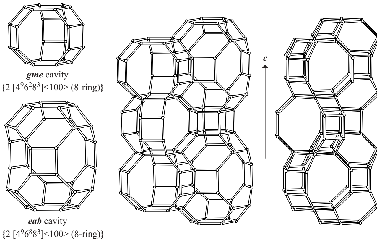
Figure 4. gme Cavity (top left) and eab cavity (bottom left) viewed along \langle 010 \rangle , fused cages viewed along \langle 010 \rangle (middle) and channels seen along \langle 100 \rangle (right).
